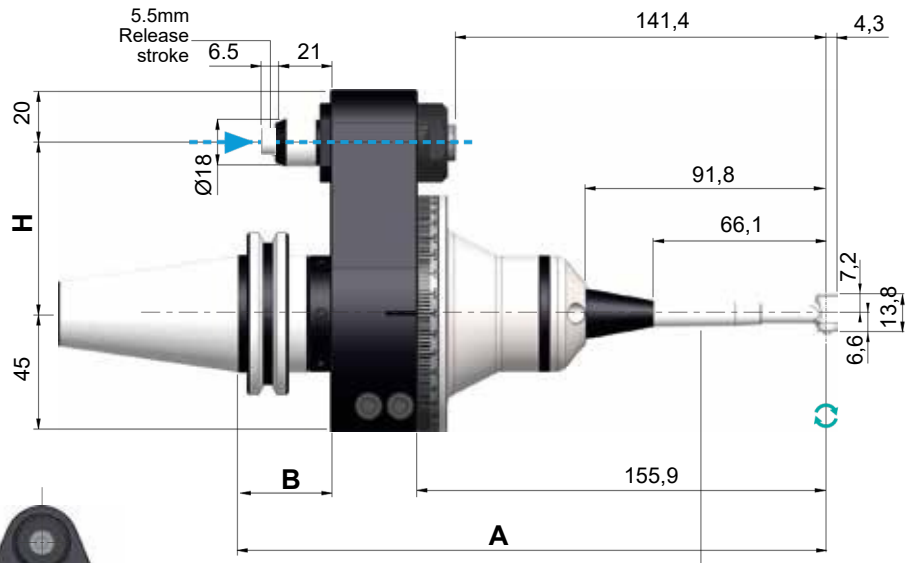
90° ANGLE SPINDLE MFC - 300 S
